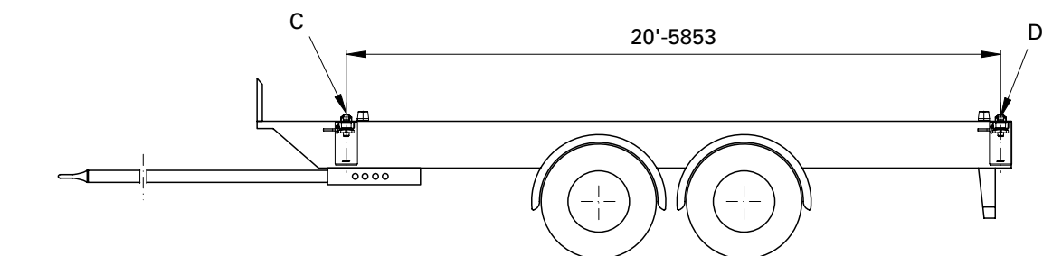
Installation examples for Intermodal vehicle / trailer
